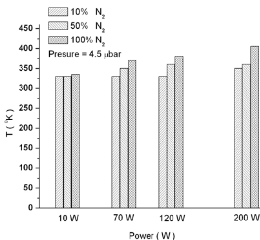
Fig.3 Gas temperatures
