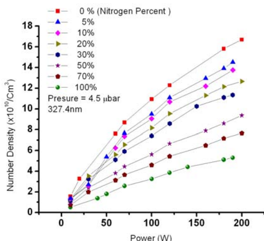
Fig. 4 \text{Cu}(^2\text{S}_{1/2} \leftarrow ^2\text{P}_{1/2}) atoms density for 4.5\mu\text{bar}
