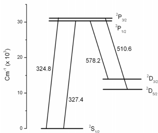
Fig. 1 Energy levels of Cu atom
