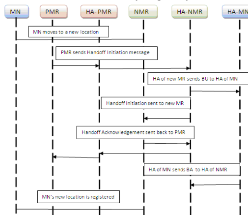
Fig. 3 Sequence diagram
