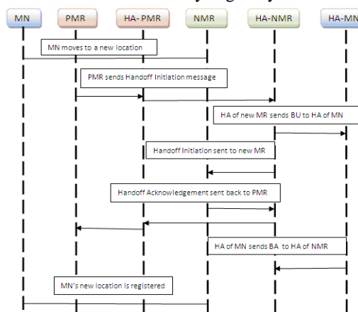
Fig. 3 Sequence diagram
