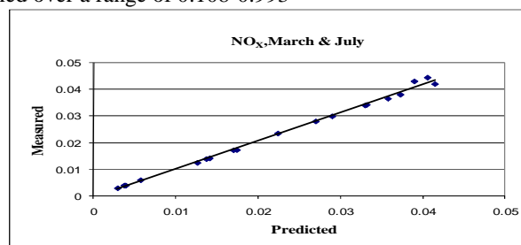
Fig. 3 Measured and Predicted concentrations of NO x
