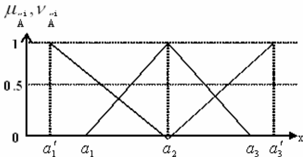
Fig. 2 Membership and non-membership functions of TIFN
