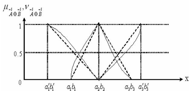
Fig. 3 Membership function of Intuitionistic fuzzy number \tilde{A} \otimes \tilde{B}
