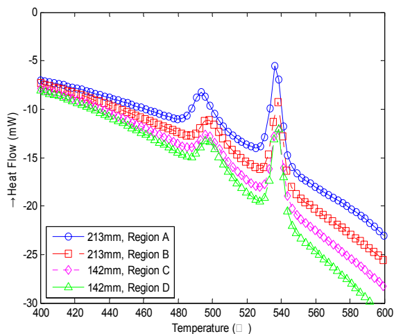
Fig. 4 DSC curves of different ribbon samples
