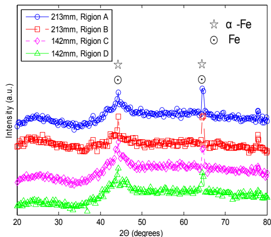
Fig. 5 XRD measured results of different ribbon samples
