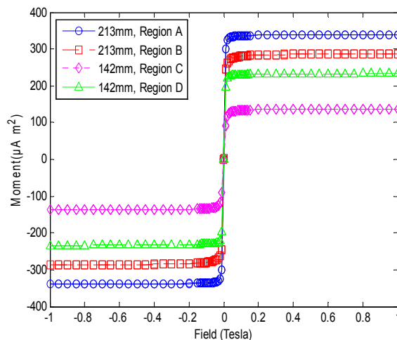
Fig. 7 The measured results of magnetic properties identified by VSM
