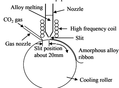
Fig. 1 Scheme diagram of single-roller rapid solidification technique
