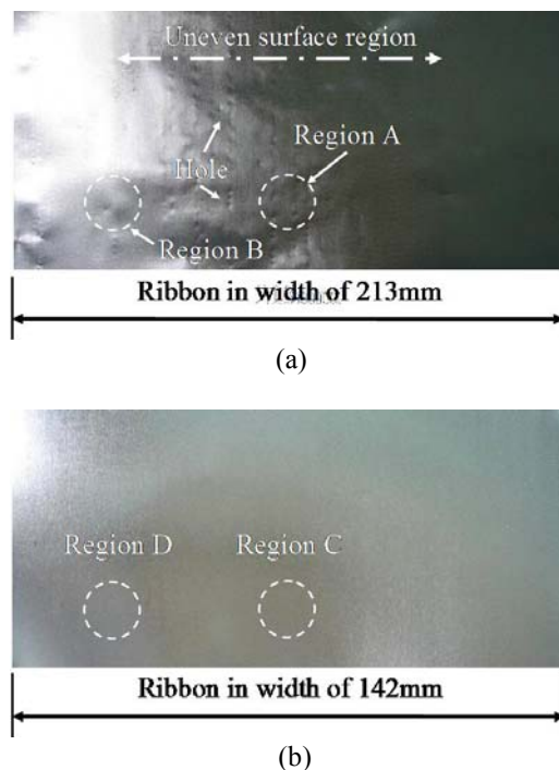
Fig. 2 Photographs of amorphous alloy ribbons in different widths: (a) 213 mm, (b) 142 mm.
