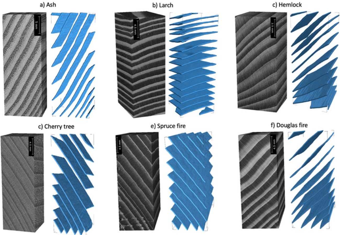
Fig. 3 The measured X-CT image stack and their calculated 3D tree-ring surfaces (plots in blue) for each wood specie studied
