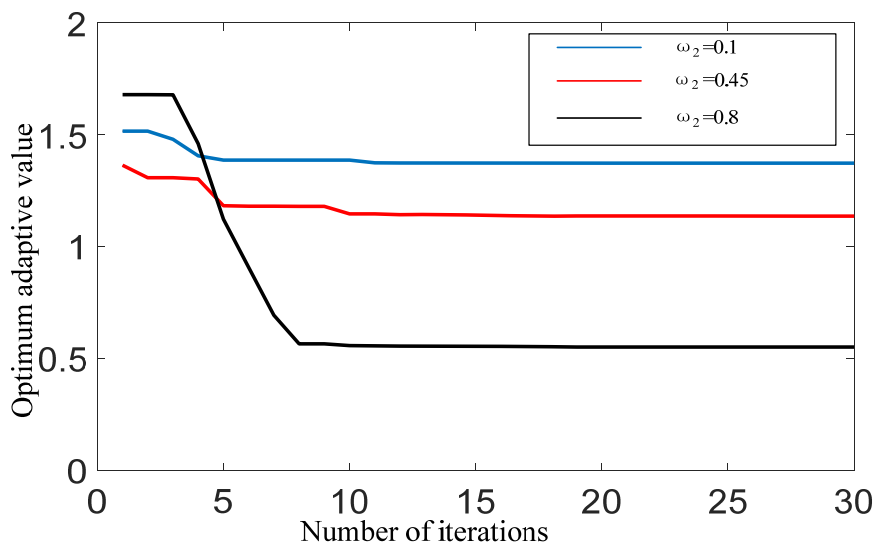
Fig. 6 Optimization curve
