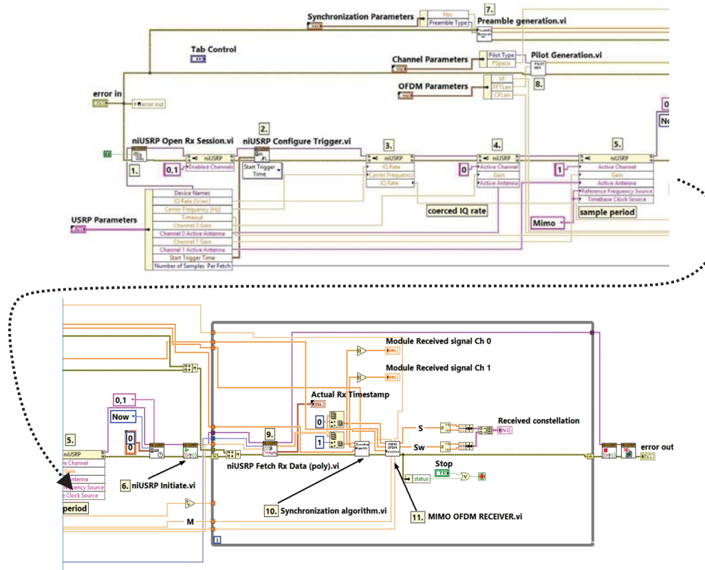
Fig. 8 The LabVIEW block diagram of 2 × 2 MIMO-OFDM Receiver
