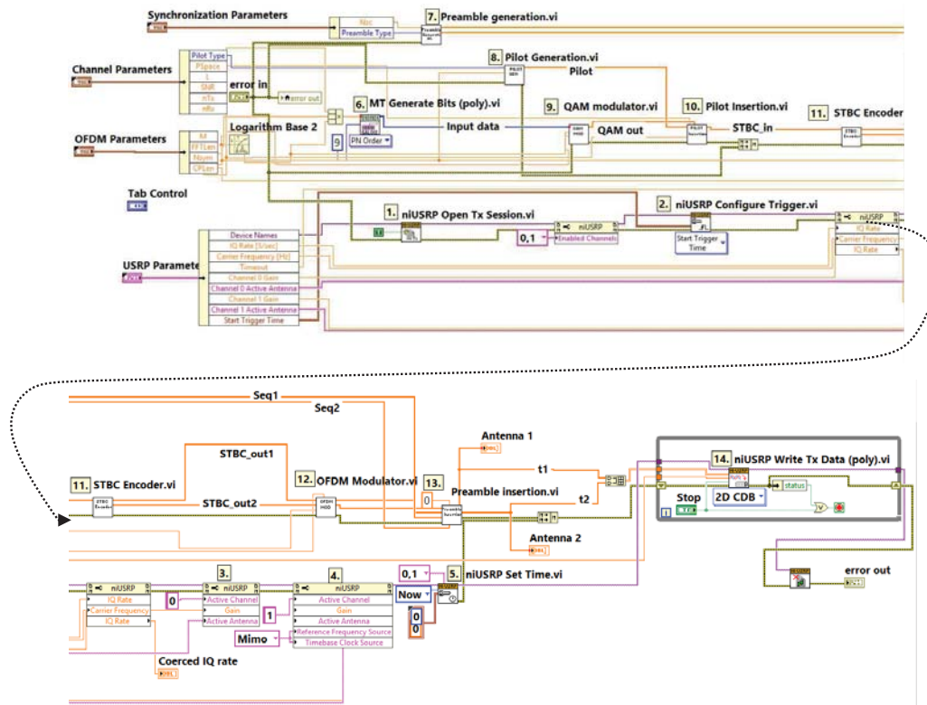
Fig. 7 The LabVIEW block diagram of 2 × 2 MIMO-OFDM Transmitter
