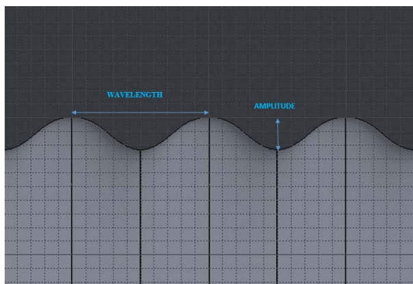
Fig. 2 The tubercles on the wing with the amplitude A = 0.06c and \lambda = 0.50c
