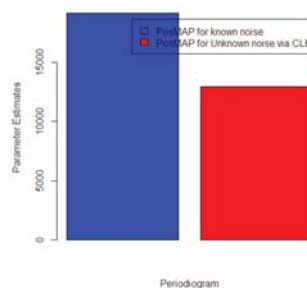
Fig. 5 Posterior Maximum A Posteriori for the Known and Unknown Noisy Sinusoidal model
