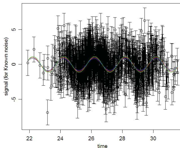
Fig. 6 Predicted 0 C for periodogram Model Unknown and Known Noise
