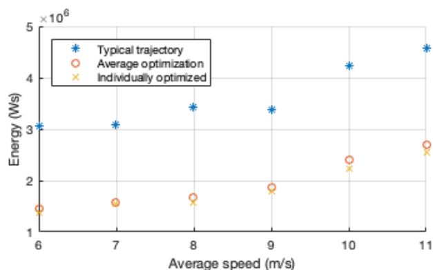
Fig. 8 Total energy spent by 10 randomly chosen vehicles in a platoon for different average speeds in a 500-meter segment.
