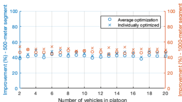
Fig. 5 Improvement in total energy spent by vehicles in a platoon for a 500m segment.
