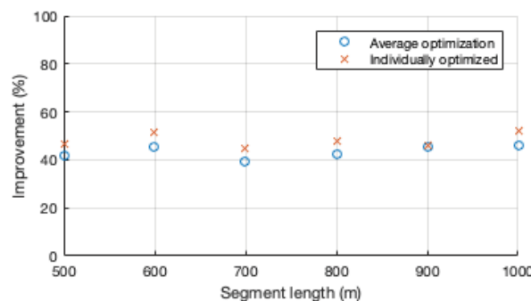
Fig. 7 Improvement in total energy spent by 10 randomly chosen vehicles in a platoon for different segment lengths with an average speed of 10 m/s.
