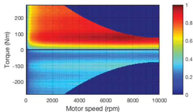
Fig. 1 Typical characterization of efficiencies.
