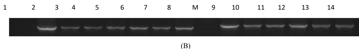
Fig. 2 A PCR products of transgenic tobacco plants that transformed with pBI-tPA-KDEL construct, amplified fragments with two primers (F-pBI and R-tPA) were 1800 bp. Lane 1 positive control, lane 2 wild type control, lanes 3-10 tobacco plants, lane M molecular ladder. B PCR products of transgenic tobacco plants that transformed with pBI-Ext-tPA and pBI-SP-tPA constructs. Amplified fragments for plants that transformed with pBI-Ext-tPA were 1900 bp, lane 1 wild type, lane 2 positive control, lanes 3-8 transgenic plants with pBI-Ext-tPA construct. M molecular ladder. Amplified fragments of the transgenic plants were 2200 bp. Lane 9 positive control, lanes 10-14 were transgenic plants
