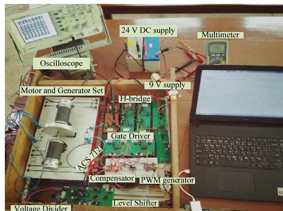
Fig. 16 Experimental Set Up with Low-Cost Hardware Implementation
