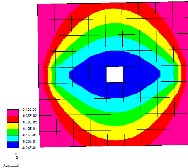
Fig. 15 The deflection mode of S3.4.4
