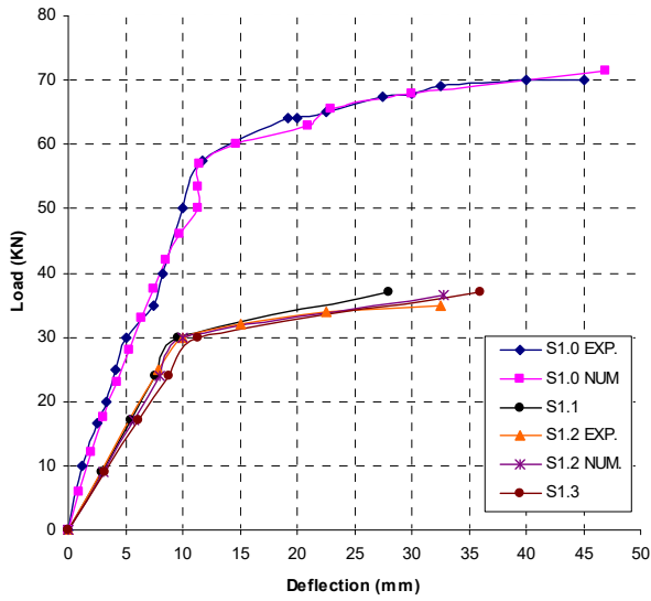
Fig. 4 Load-deflection curve of Group I
