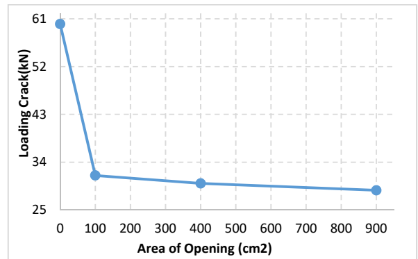
Fig. 8 The relationship between loading crack and area of opening
