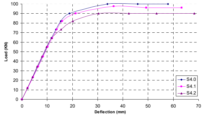
Fig. 7 Load-deflection curve of Group IV
