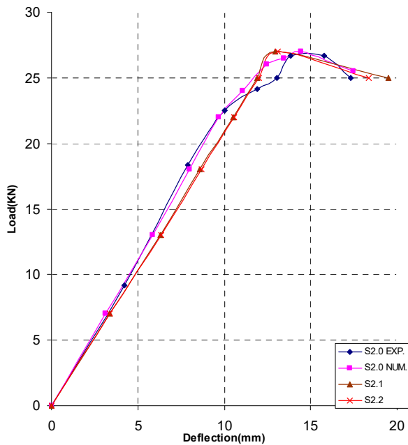
Fig. 5 Load-deflection curve of Group II
