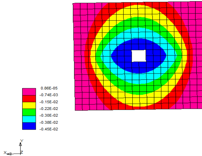
Fig. 14 The deflection mode of 3.2.2
