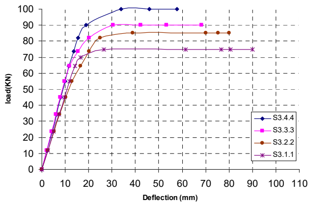
Fig. 6 Load-deflection curve of Group III
