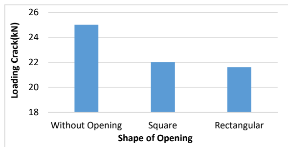
Fig. 9 The relationship between loading crack and shape of opening
