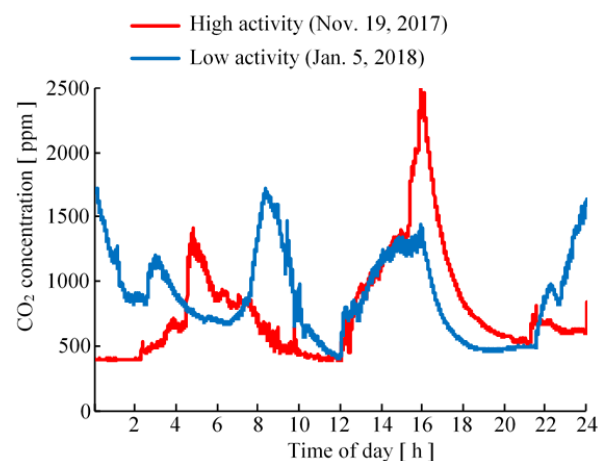
Fig. 4 CO 2 sensor outputs
