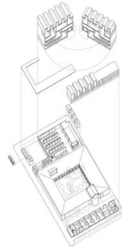
Fig. 8 Perspective design of roofing systems at the Museum of Fine Arts of Castellón [16]
