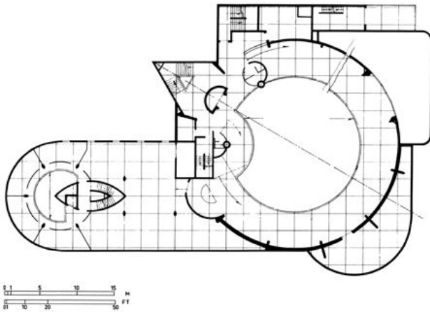
Fig. 3 The New York Guggenheim floor plan [12]
