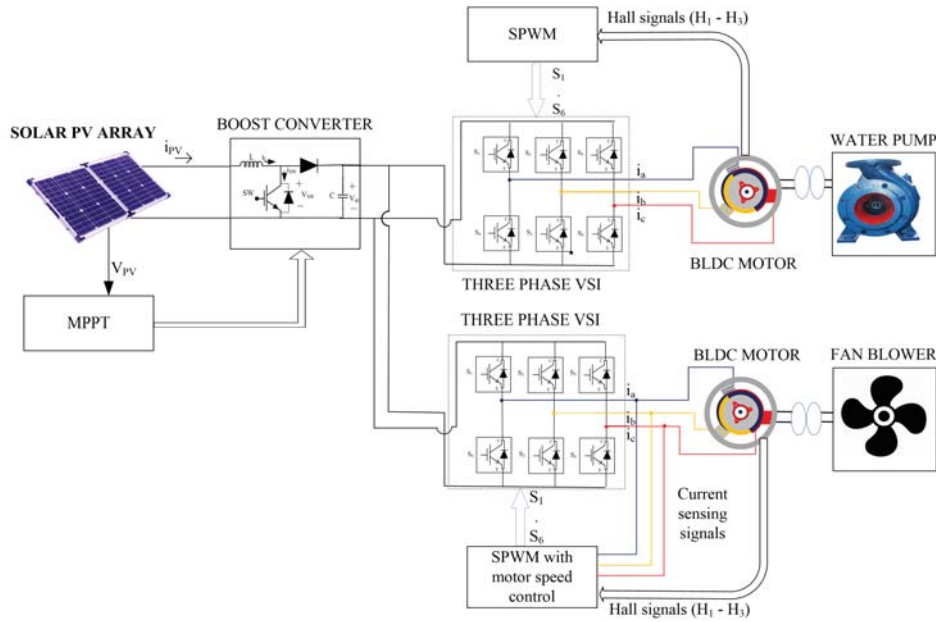
Fig. 1 Proposed SPV fed air cooling system
