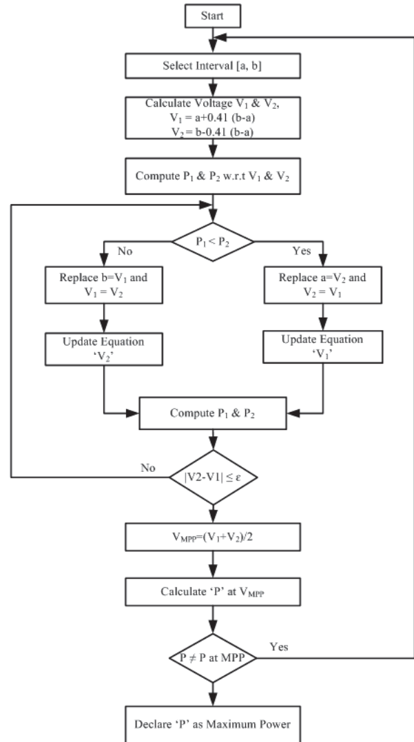
Fig. 3 Flow chart of the proposed MPPT algorithm
