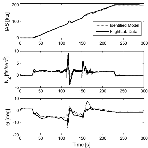
Fig. 9 Comparison between identified model outputs and simulated flight data for conversion from helicopter to aircraft: rigid body dynamics
