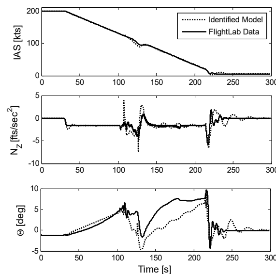
Fig. 6 Comparison between identified model outputs and simulated flight data for conversion from aircraft to helicopter: rigid body dynamics
