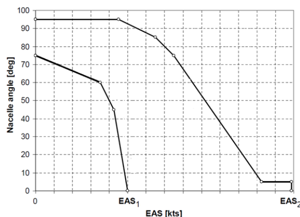
Fig. 1 Tilt-rotor conversion corridor envelope
