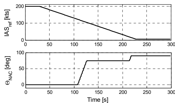
Fig. 5 Model inputs for conversion from aircraft to helicopter: time histories of reference IAS and nacelle angle
