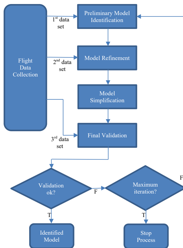
Fig. 3 Rigid Body model identification strategy
