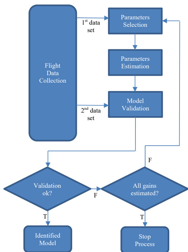
Fig. 4 Flapping model identification strategy
