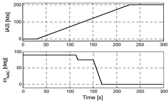
Fig. 8 Model inputs for conversion from helicopter to aircraft: time histories of reference IAS and nacelle angle
