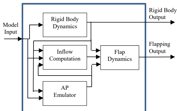
Fig. 2 Tilt-rotor model structure
