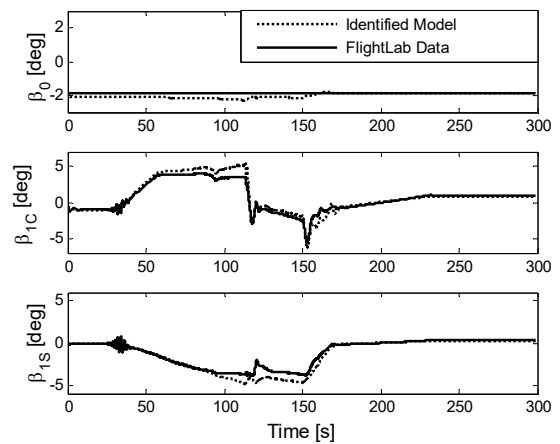
Fig. 10 Comparison between identified model outputs and simulated flight data for conversion from helicopter to aircraft: flapping dynamics
