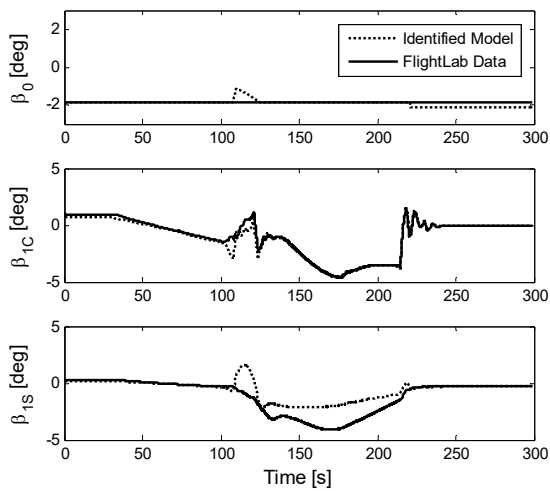
Fig. 7 Comparison between identified model outputs and simulated flight data for conversion from aircraft to helicopter: flapping dynamics
