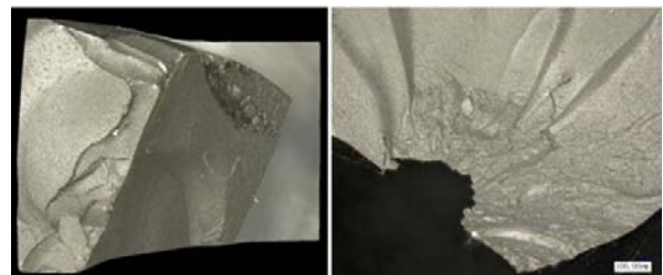
Fig. 14 Fracture of coated carbide bit
