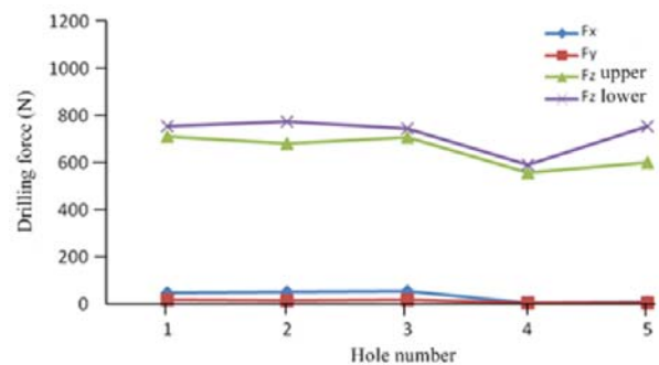
Fig. 17 Change of drilling force when the coated carbide tool was used
