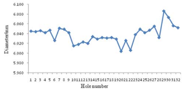
Fig. 6 Change of hole diameter
