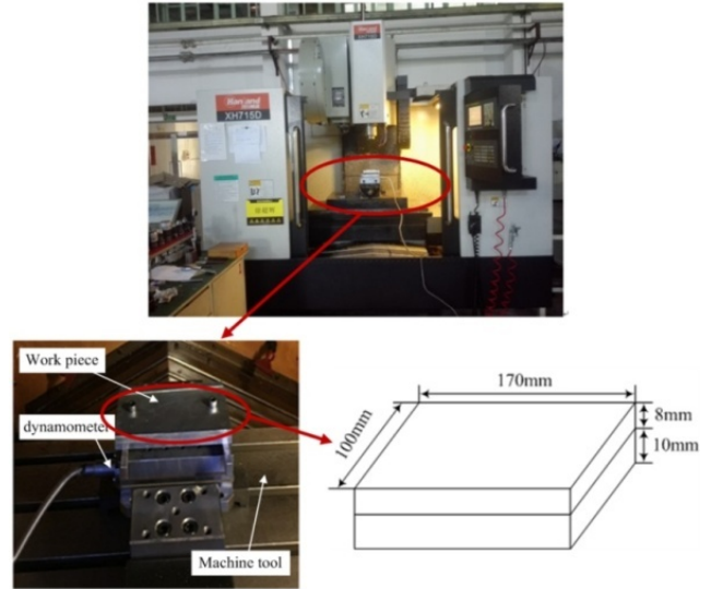
Fig. 1 Experiment device and work-piece
