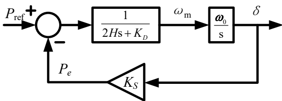
Fig. 3 Transfer function block diagram of the VSG
