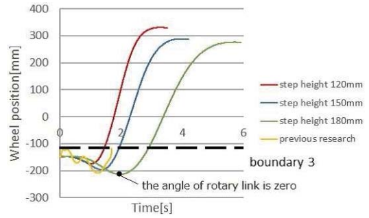
Fig. 14 Time history of the lower wheels position during the wheel-linkage control stage
