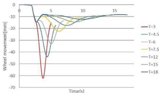
Fig. 9 Relationship between wheel movement and the period for per step
