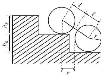
Fig. 8 Wheels and stairs
