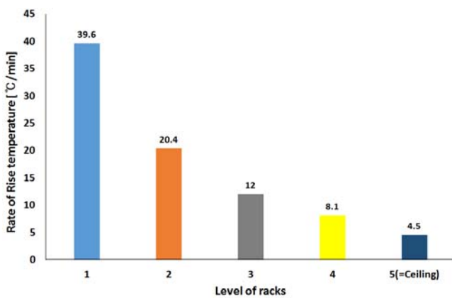
Fig. 9 The rate of temperature rise per minute
