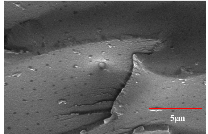
Fig. 11 SEM image of monolithic polyester exposed in water-methanol
