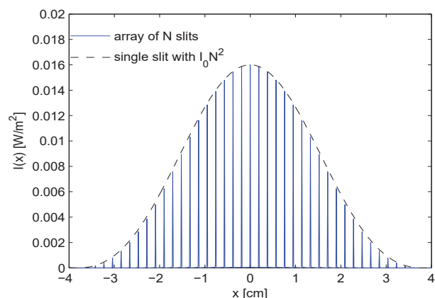
Fig. 2 Intensity pattern I(x) of uniform diffraction grating, N = 20
