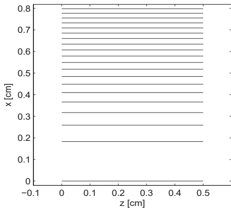
Fig. 7 Prototype of aperiodic diffraction grating, N = 20
