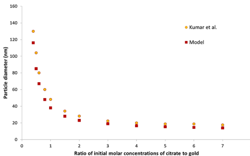
Fig. 1 The model predictions in Parsival compared to those of Kumar et al. [7]
