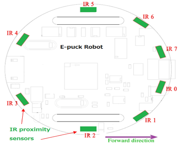
Fig. 8 E-puck robot proximity sensors
