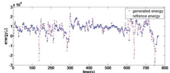
Fig. 10 Tracking reference energy by generated energy through the HWYCOL drive cycle
