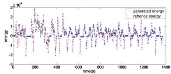
Fig. 9 Tracking reference energy by generated energy through the UDSS drive cycle
