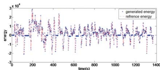
Fig. 9 Tracking reference energy by generated energy through the UDSS drive cycle
