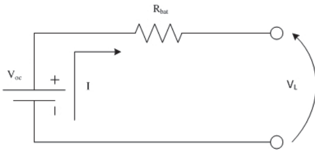
Fig. 2 Electric circuit of the battery
