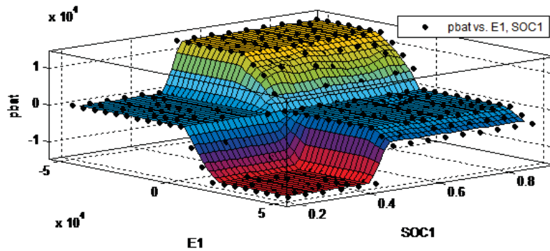
Fig. 5 P_{bat} vs E_1 and SOC_1 while SOC_r = 0.5 and E_r = 0J
