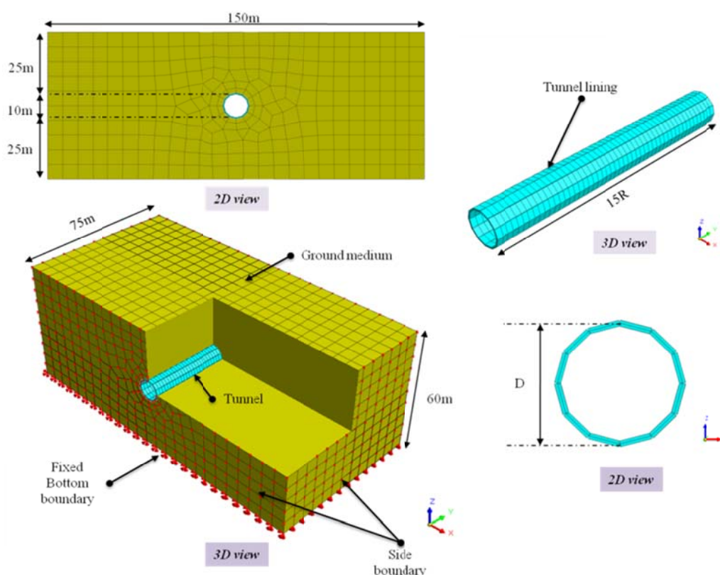
Fig. 2 Geometry, meshing and boundary conditions of the soil-tunnel system
