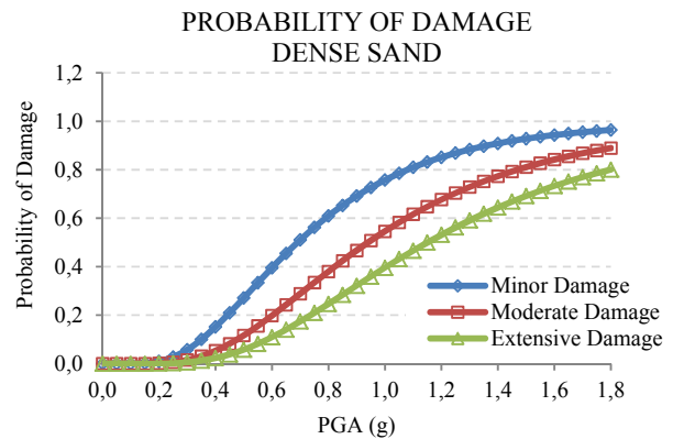
Fig. 8 Fragility curves of circular tunnel for dense sand
