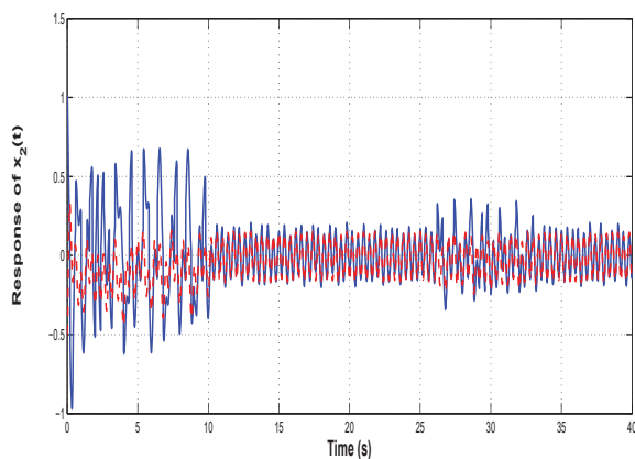
Fig. 3 Response of x_2(t) (solid line) and its estimate \hat{x}_2(t) (dashed line)
