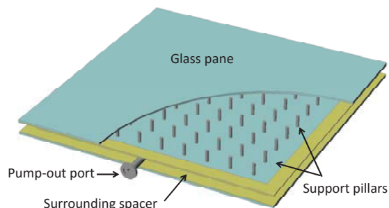
Fig. 8 Schematic diagram of a flat vacuum panel
