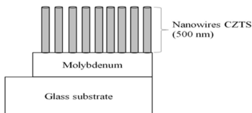
Fig. 5 Nanowires development in CZTS [16]
