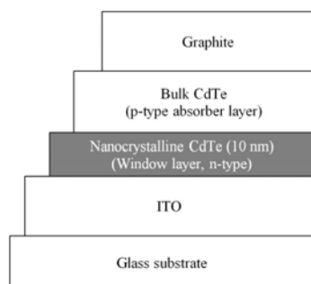
Fig. 1 Nanocrystalline development in CdTe Solar Cell [11]
