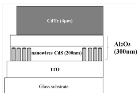
Fig. 2 Nanowires development in CdTe Solar cell [12]
