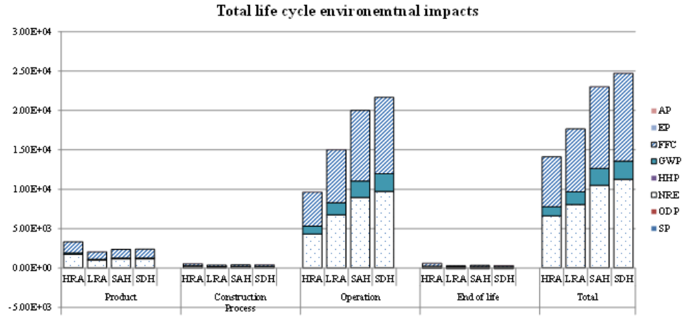
Fig. 8 Total life-cycle environmental Impacts
