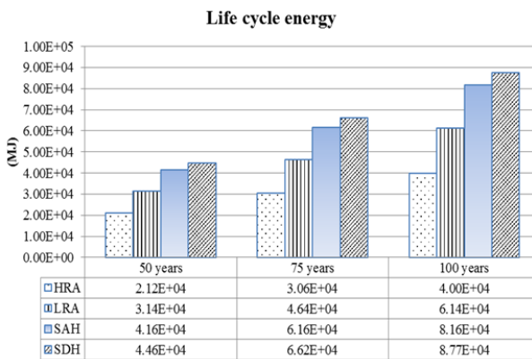
Fig. 9 Life cycle energy for residential buildings
