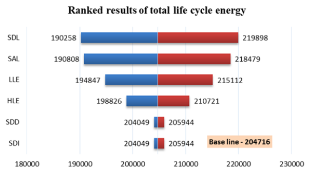
Fig. 11 Sensitivity analysis for total life-cycle energy
