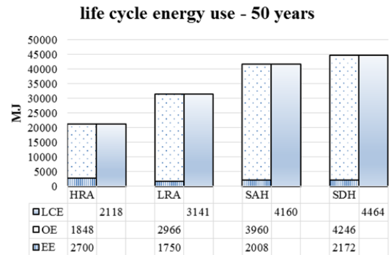
Fig. 7 Total life cycle energy use for 50-years lifespan
