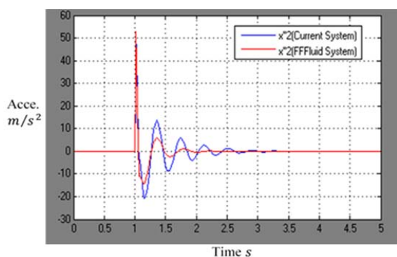
Fig. 9 Ride comfort
