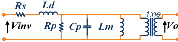
Fig. 2 Equivalent lumped parameters transformer model
