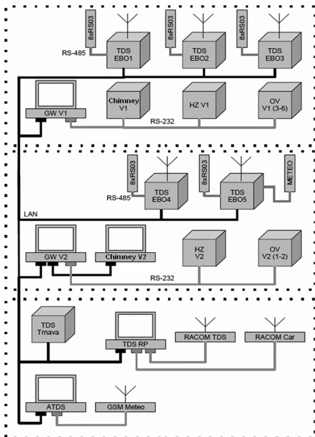
Fig. 1 Today's structure of the teledosimetric system
