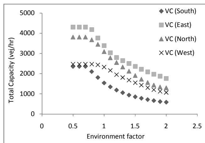
Fig. 7 Effect of Environment Factor on total capacity
