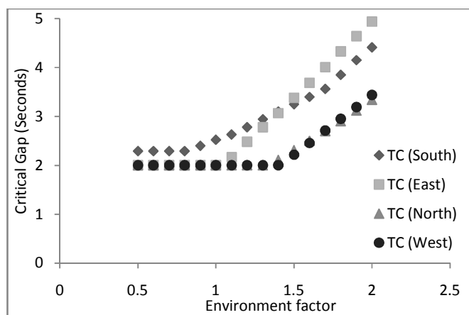
Fig. 4 Effect of Environment Factor on critical gap
