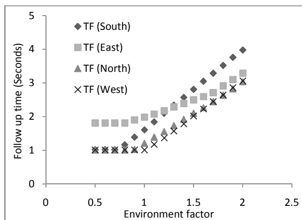
Fig. 5 Effect of Environment Factor on follow up time
