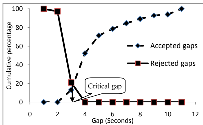
Fig. 3 Critical gap for North Approach
