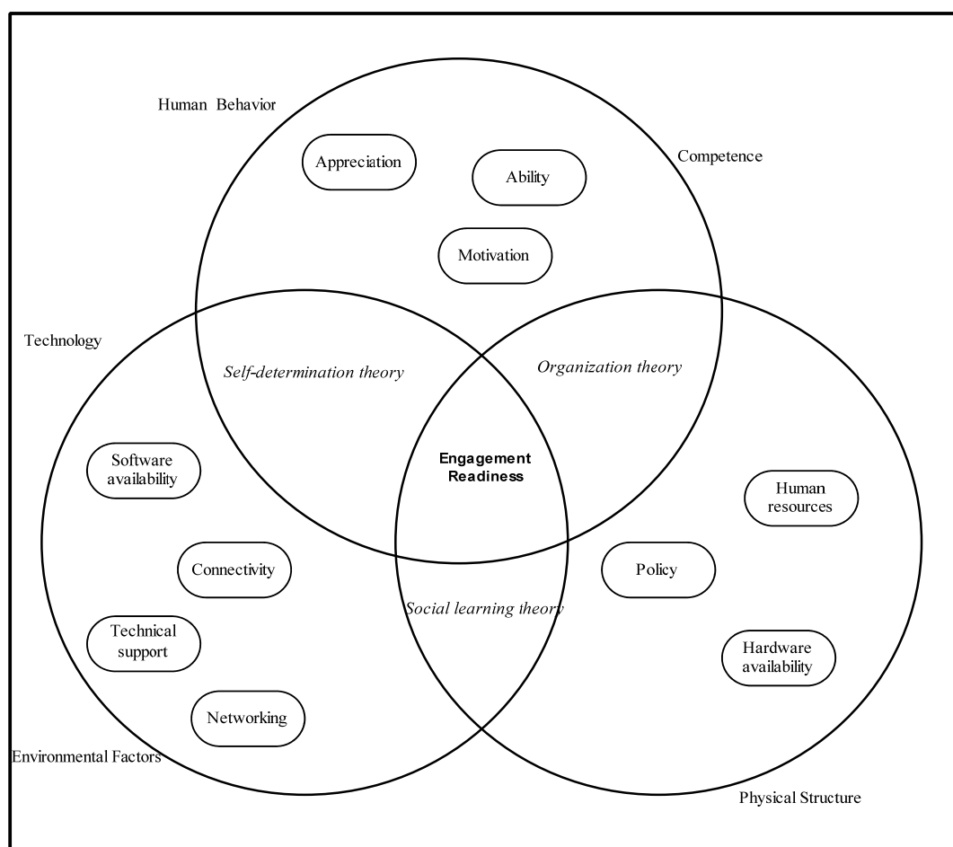
Fig. 1 Theoretical framework
