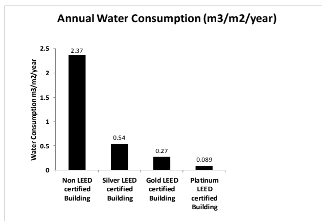
Fig. 7 Annual water consumption of studied buildings
