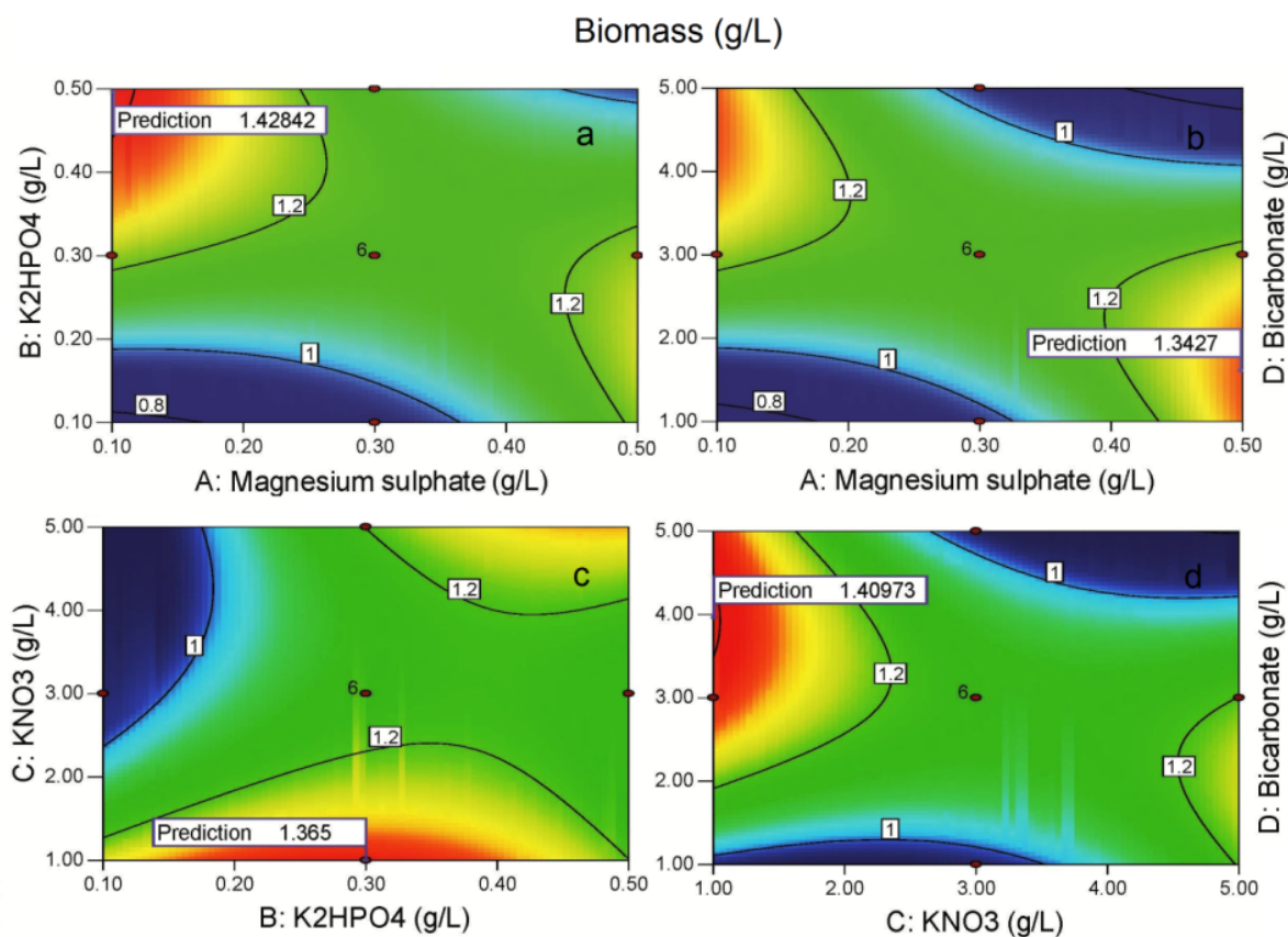
Fig. 1 Contour plots representing biomass yield from culture of C. pyrenoidosa as affected by cultural conditions (a) K 2 HPO 4 and MgSO 4 (b) NaHCO 3 and MgSO 4 (c) KNO 3 and K 2 HPO 4 (d) NaHCO 3 and KNO 3 . All the values expressed in terms of g/L.
