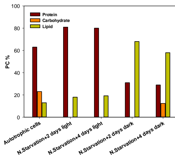
Fig. 3 The cellular variability of C. pyrenoidosa in terms of protein, carbohydrate and lipid content under N stress conditions on day 2 and day 4. PC refers to Principal Components derived from the data analysis of peak area integration from FTIR
