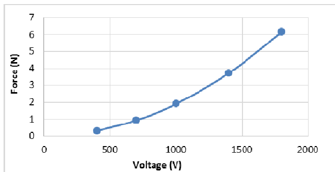
Fig. 7 Graph of adhesive force and voltage
