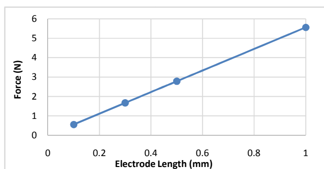
Fig. 12 Attraction force compared to the electrodes length
