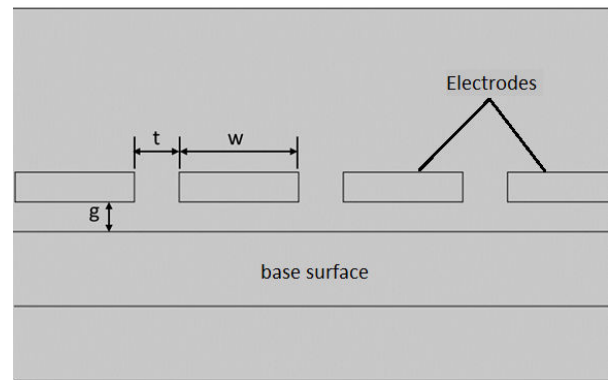
Fig. 5 Parameters in the Two-dimensional model
