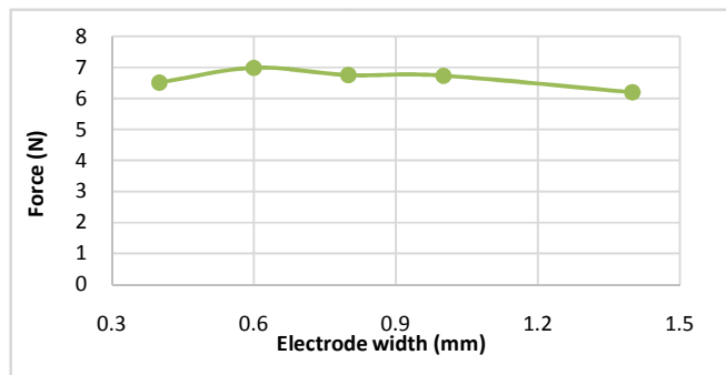
Fig. 9 The adhesive force compared to width of the electrodes
