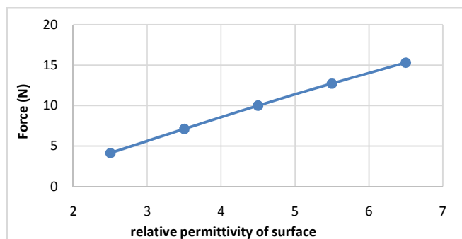
Fig. 10 Adhesion force compared to the surface Relative permittivity
