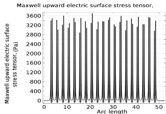
Fig. 6 Stress on the surface
