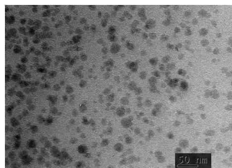
Fig. 6 TEM image of a grafted PS-silica composite
