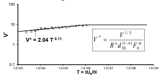
Fig. 13 Proposed scaling variables on volume of scour
