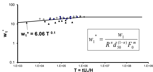
Fig. 14 Proposed scaling variables on maximum ridge width
