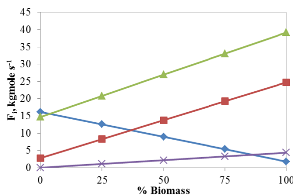
Fig. 6 Distribution of the three major species in independent co-gasification process
