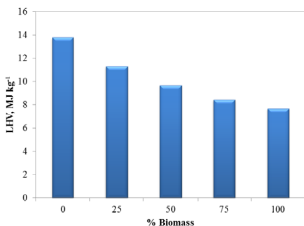
Fig. 5 Heating values for the produced raw syngas
