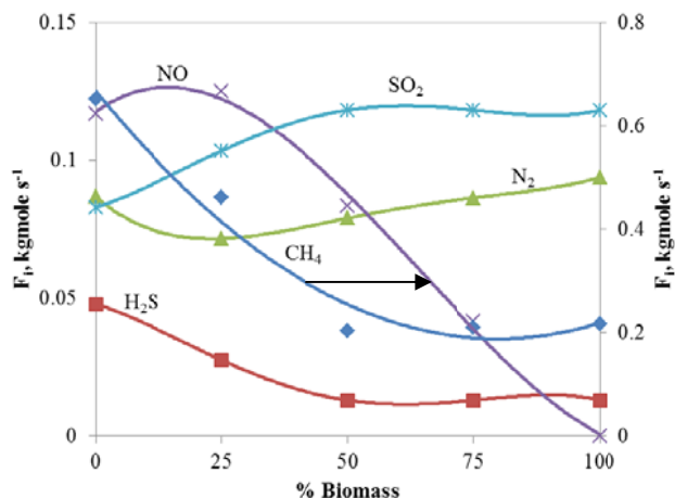
Fig. 4 Minor species molar flow with increasing biomass content
