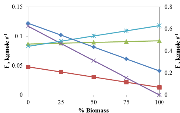
Fig. 7 Distribution of the minor species in independent co-gasification process
