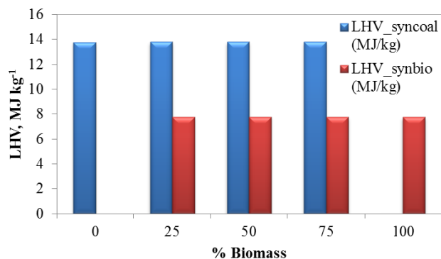
Fig. 8 The LHV of the produced syngas with increasing biomass percentage
