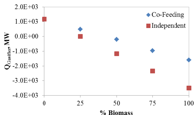
Fig. 9 Heat generated or consumed in the gasifiers with increasing biomass content
