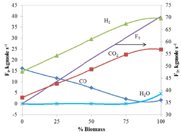
Fig. 3 Total and major species molar flow with increasing biomass content
