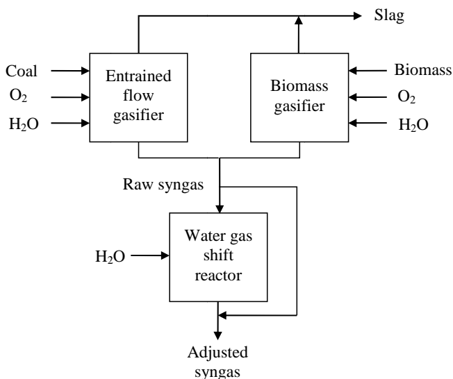
Fig. 2 Schematic diagram for independent co-gasification process
