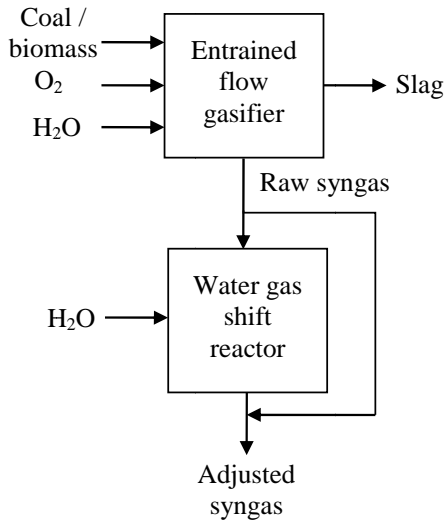
Fig. 1 Schematic diagram for co-feeding configuration for co-gasification process
