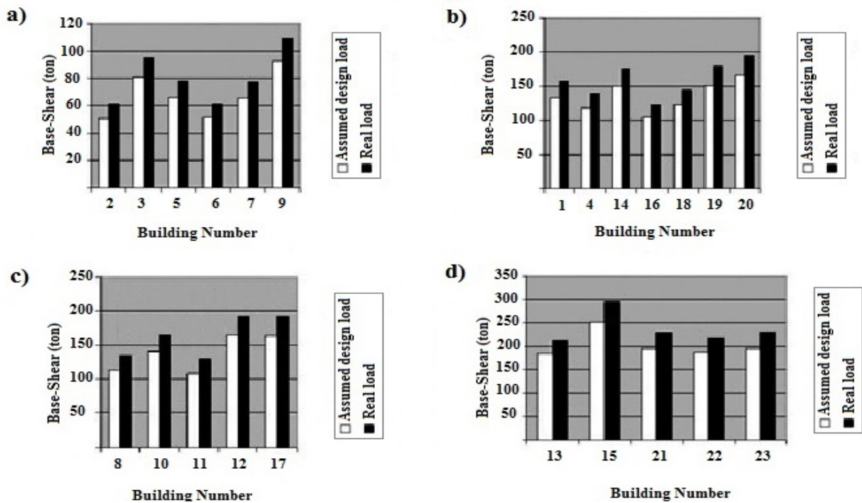
Fig. 3 Comparison between base-shears of buildings with assumed design loads and real loads in construction (Groups a, b, c, d)
