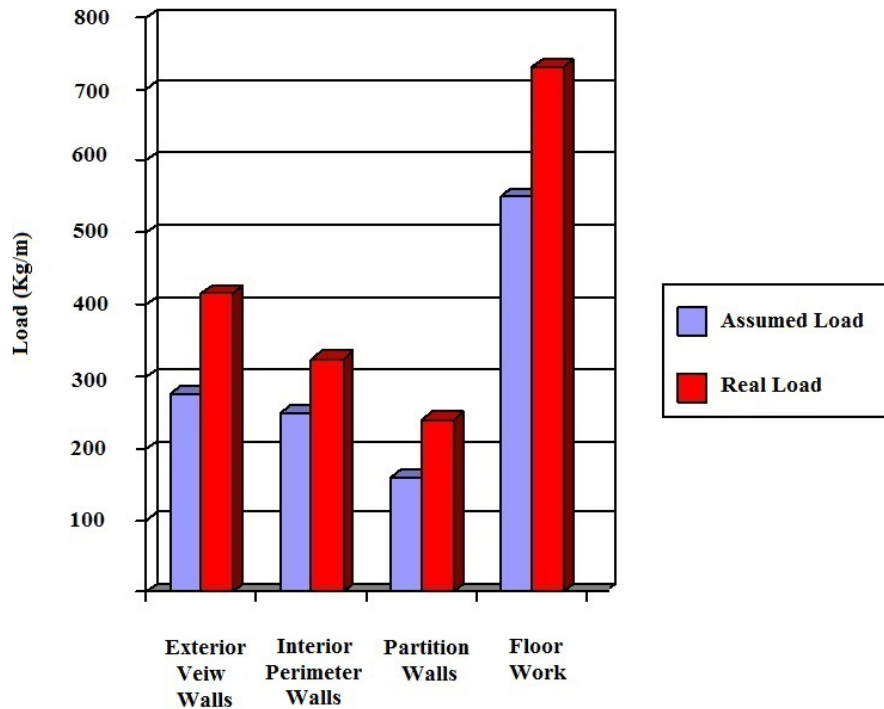
Fig. 2 Comparison between assumed loads in design and real loads in construction
