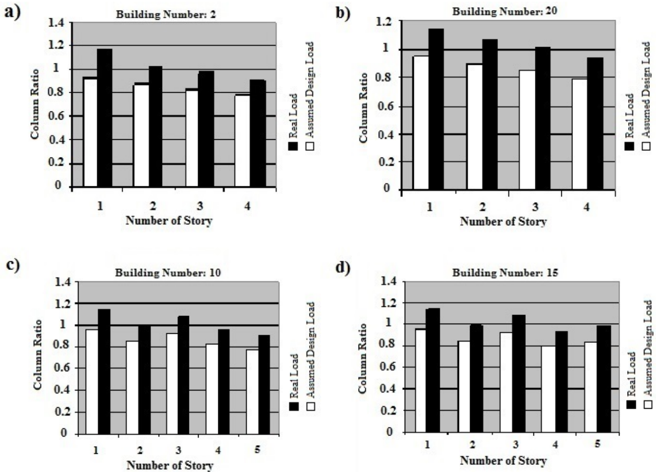
Fig. 5 Stresses ratio for the most critical exterior column of a building in groups a, b, c, d
