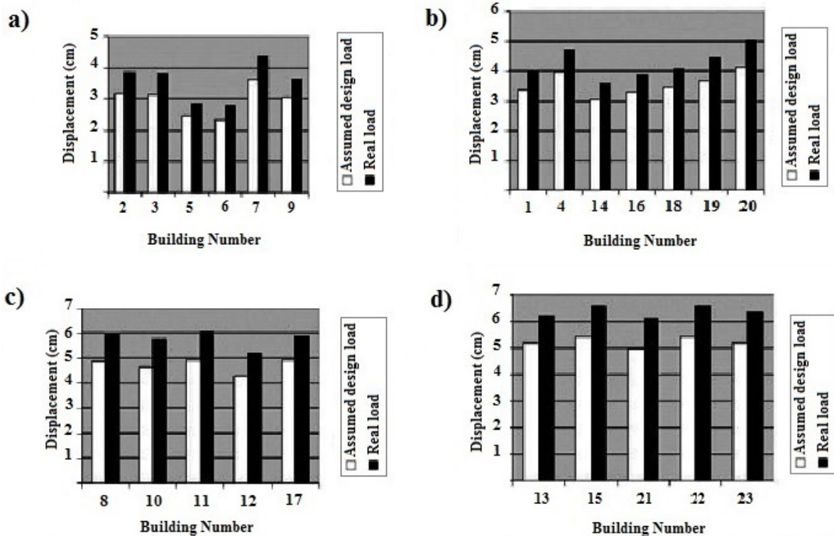
Fig. 4 Comparison between roof-floor displacements of buildings with assumed design loads and real loads in construction (Groups a, b, c, d)
