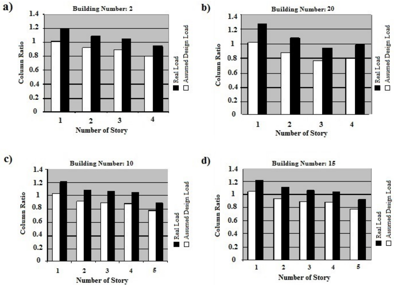
Fig. 6 Stresses ratio for the most critical interior column of a building in groups a, b, c, d
